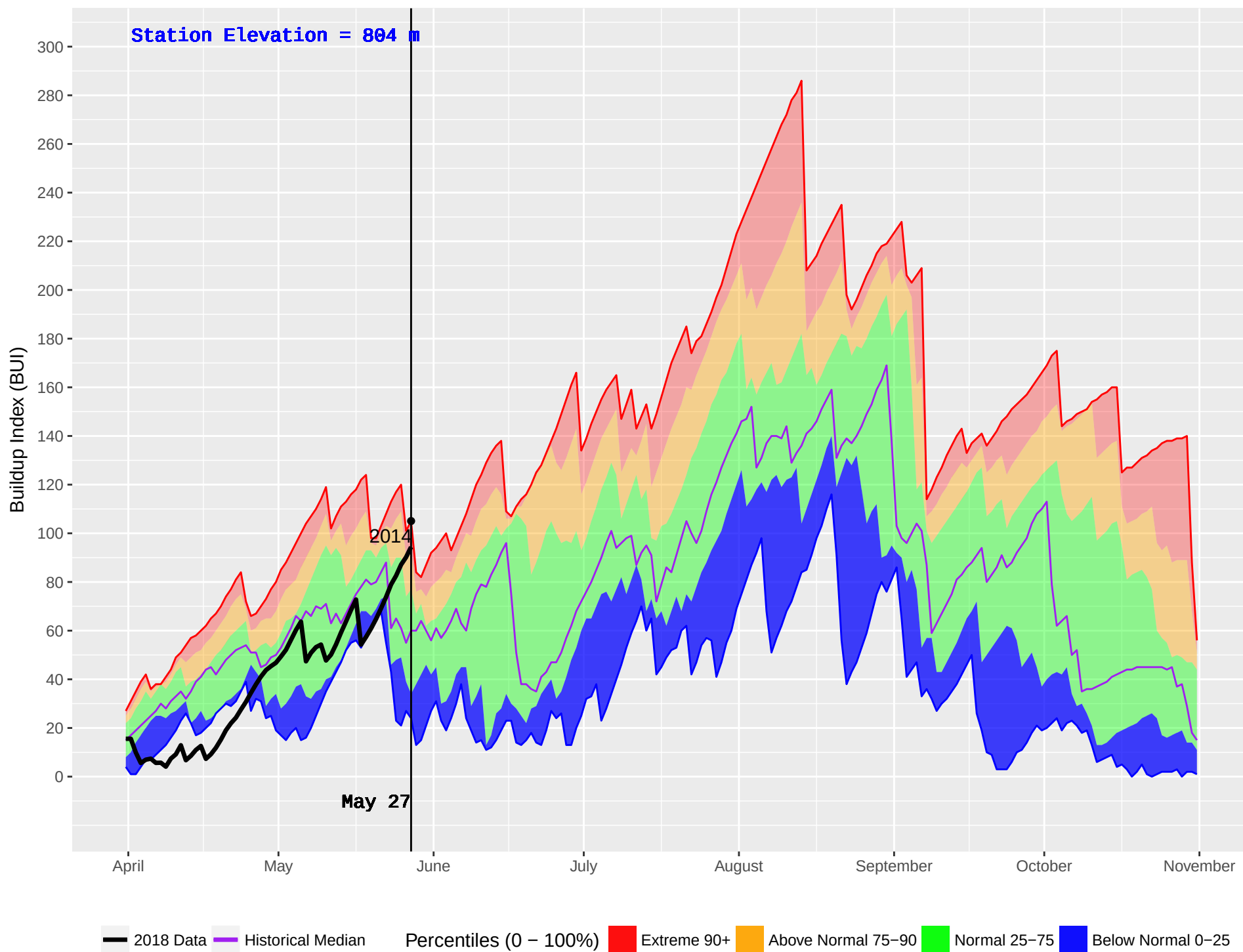
KOOCANUSA (1075) : Historical (2010–2016) and Current (2018) Noon Buildup Index (BUI)
